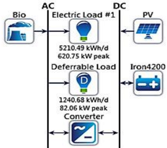
Figure 3: Design Schematics
