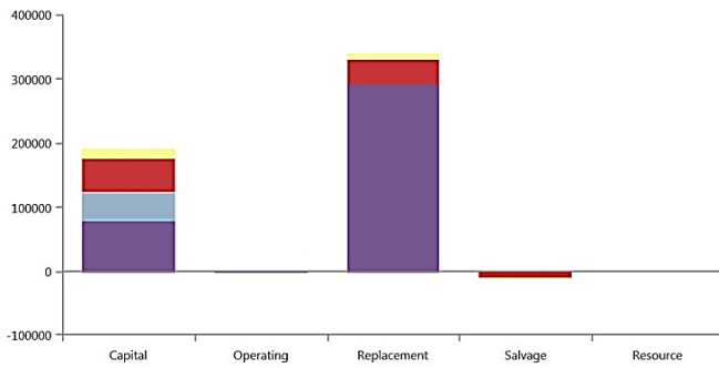
Figure 5: Cost Summary of Optimal System
